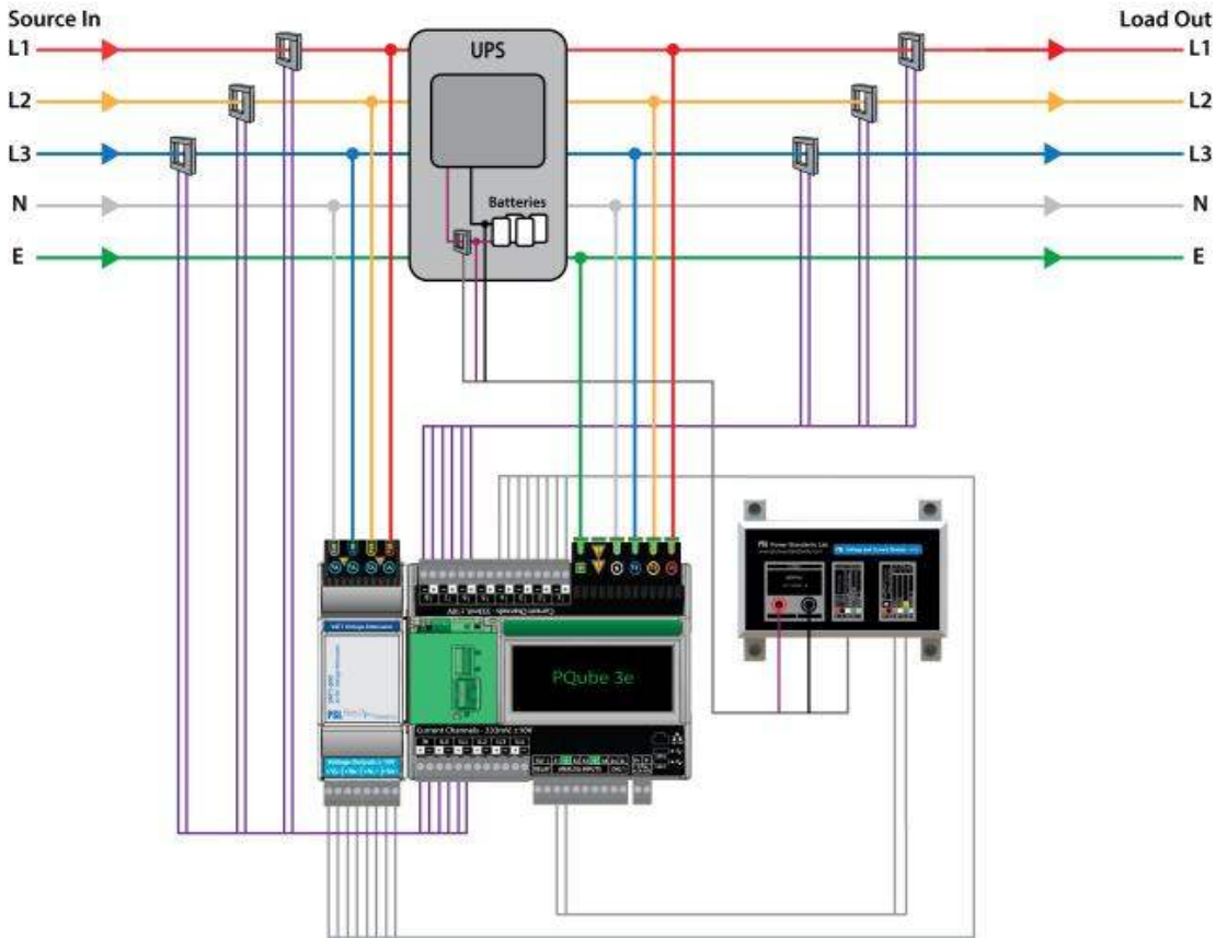
Wiring Diagram: UPS Monitoring
