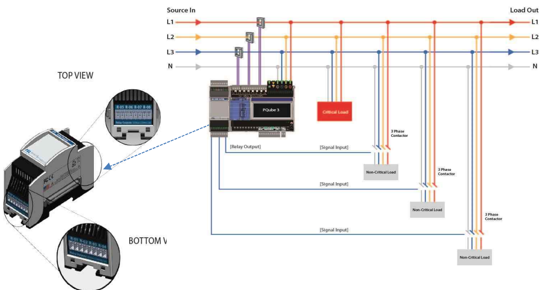
WIRING FOR MONITORING WITH ONE 3-PHASE LOAD
